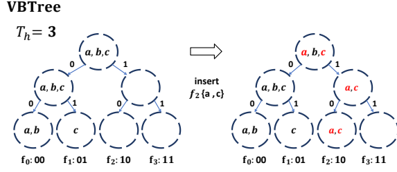
Fig. 1. An example of vbtree.
